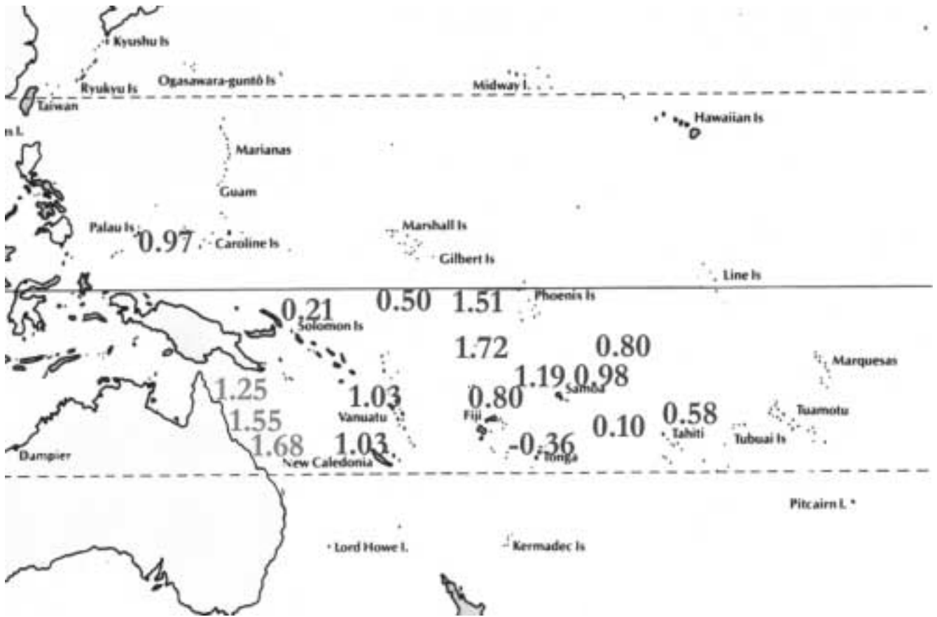
Figure 4. Map showing relative position of rates of sea temperature warming over the 1900s for 17 Pacific locations. Rates of warming calculated by Hoegh-Guldberg (1999) for data from three sites on the Great Barrier Reef are shown in light grey type.
